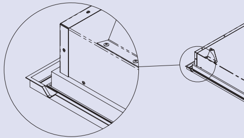
Type PGL2/T Tegular Ceiling
