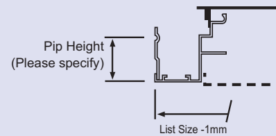
Type PGL2/B Clip in Ceiling
