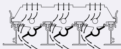
HORIZONTAL DISTRIBUTION - 2 way Airflow
